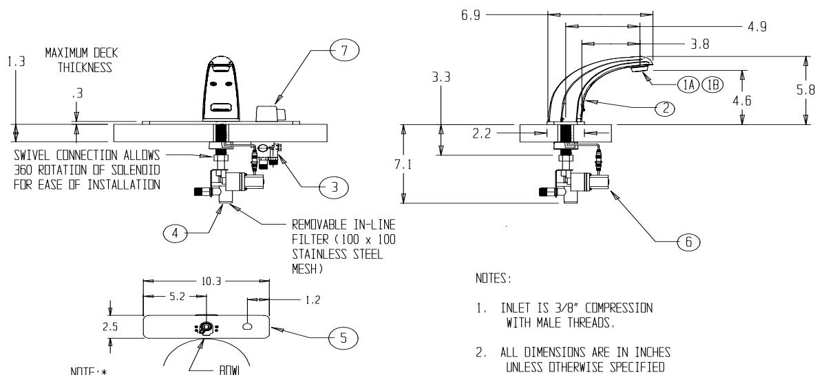
S-8722 SERIES
